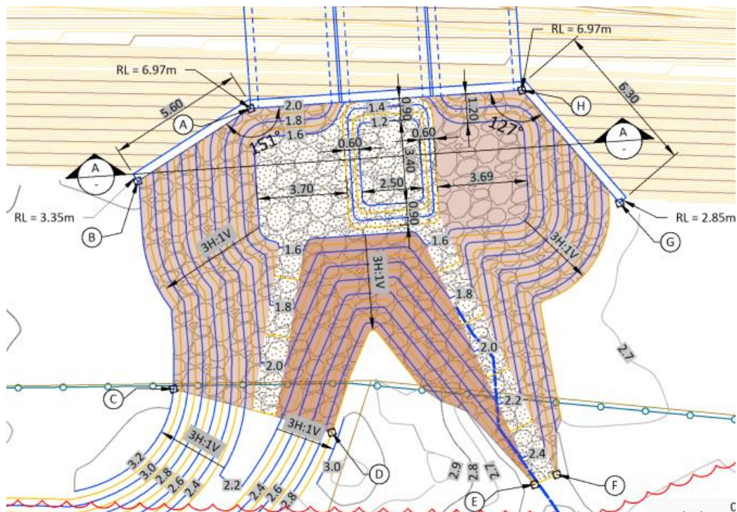
Figure 4-14: Plan view of upstream apron with stream and steep tributary confluence.
