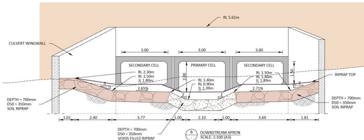
Figure 4-13: Cross-section of scour-protected apron for large triple box culvert. Designed for 100-Year climate-adjusted flows and fish passage at ½ of 2-year ARI flow.
