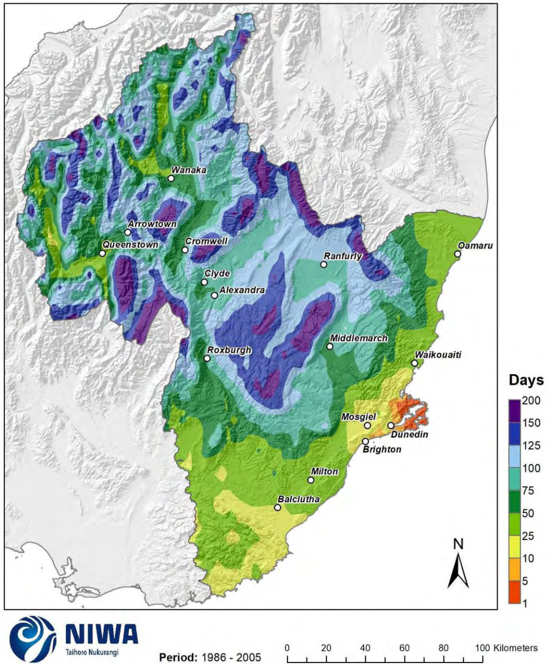
Figure 3-26: Modelled annual number of frost days (daily minimum temperature <math><0^{\circ}\text{C}</math>), average over 1986-2005. Results are based on dynamical downscaled projections using NIWA's Regional Climate Model. Resolution of projection is 5km x 5km.
