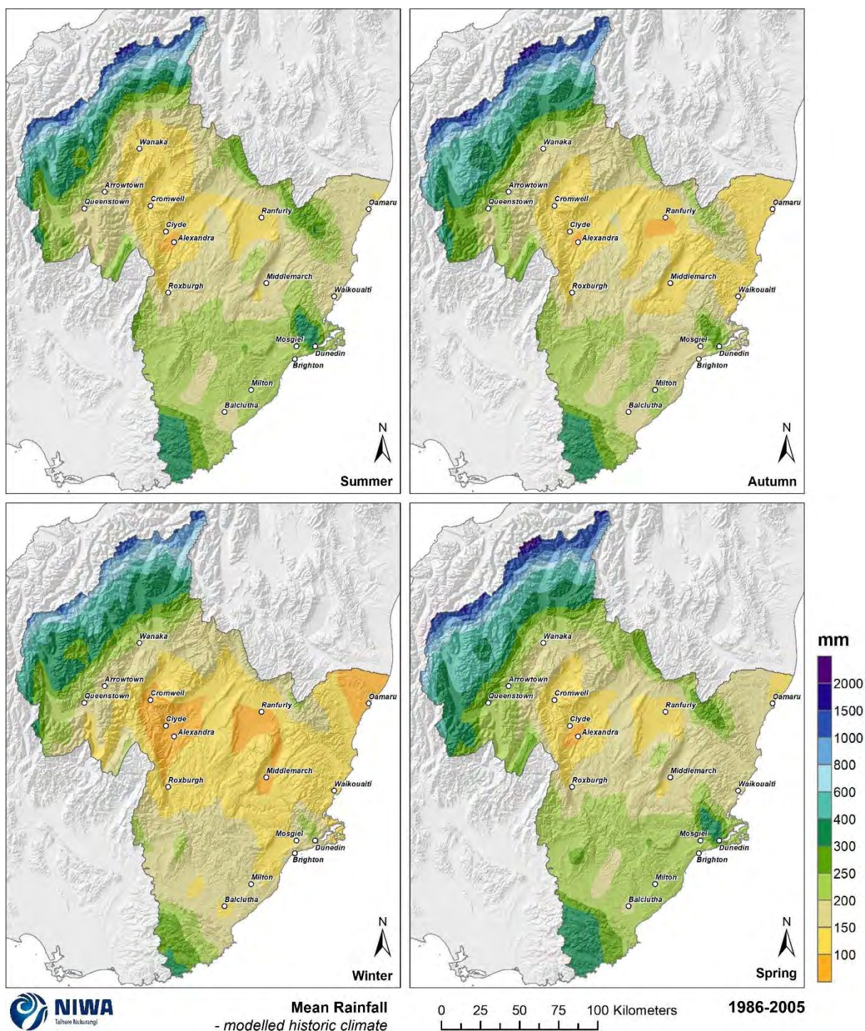
Figure 4-3: Modelled seasonal mean rainfall, average over 1986-2005. Results are based on dynamical downscaled projections using NIWA's Regional Climate Model. Resolution of projection is 5km x 5km.
