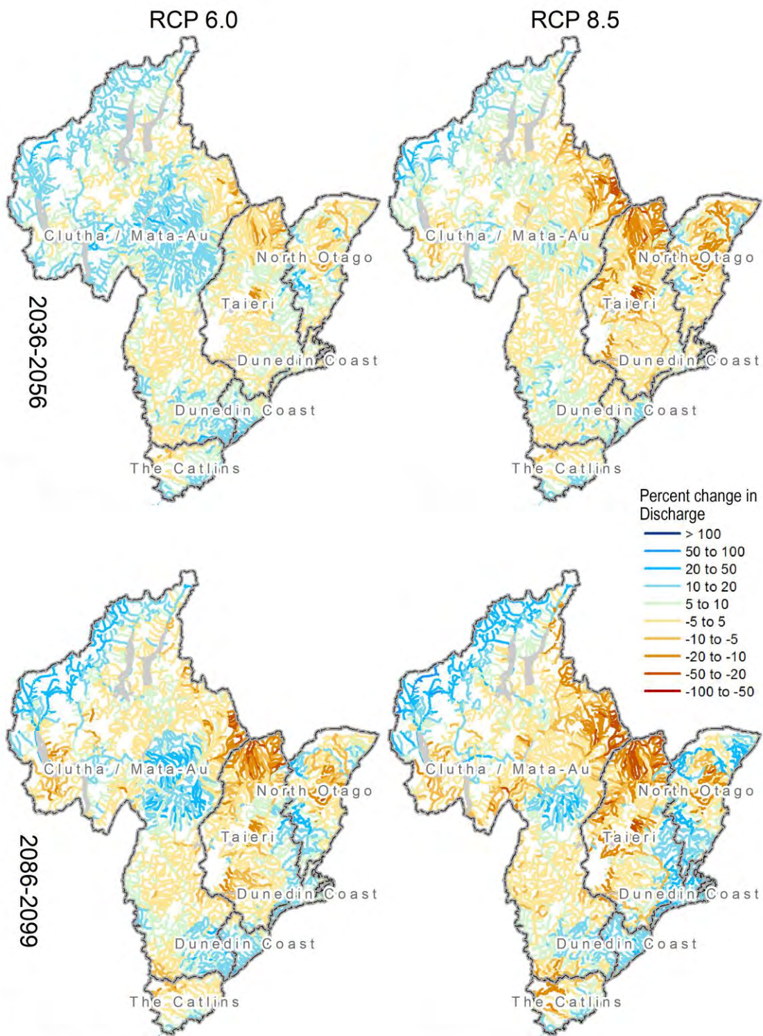
Figure 6-2: Percent changes in multi-model median Q95 across Otago for mid (top) and end of century (bottom). Climate change scenarios: RCP6.0 (left panels) and RCP8.5 (right panels). Time periods: mid-century (2036-2056) and end-century (2086-2099).
